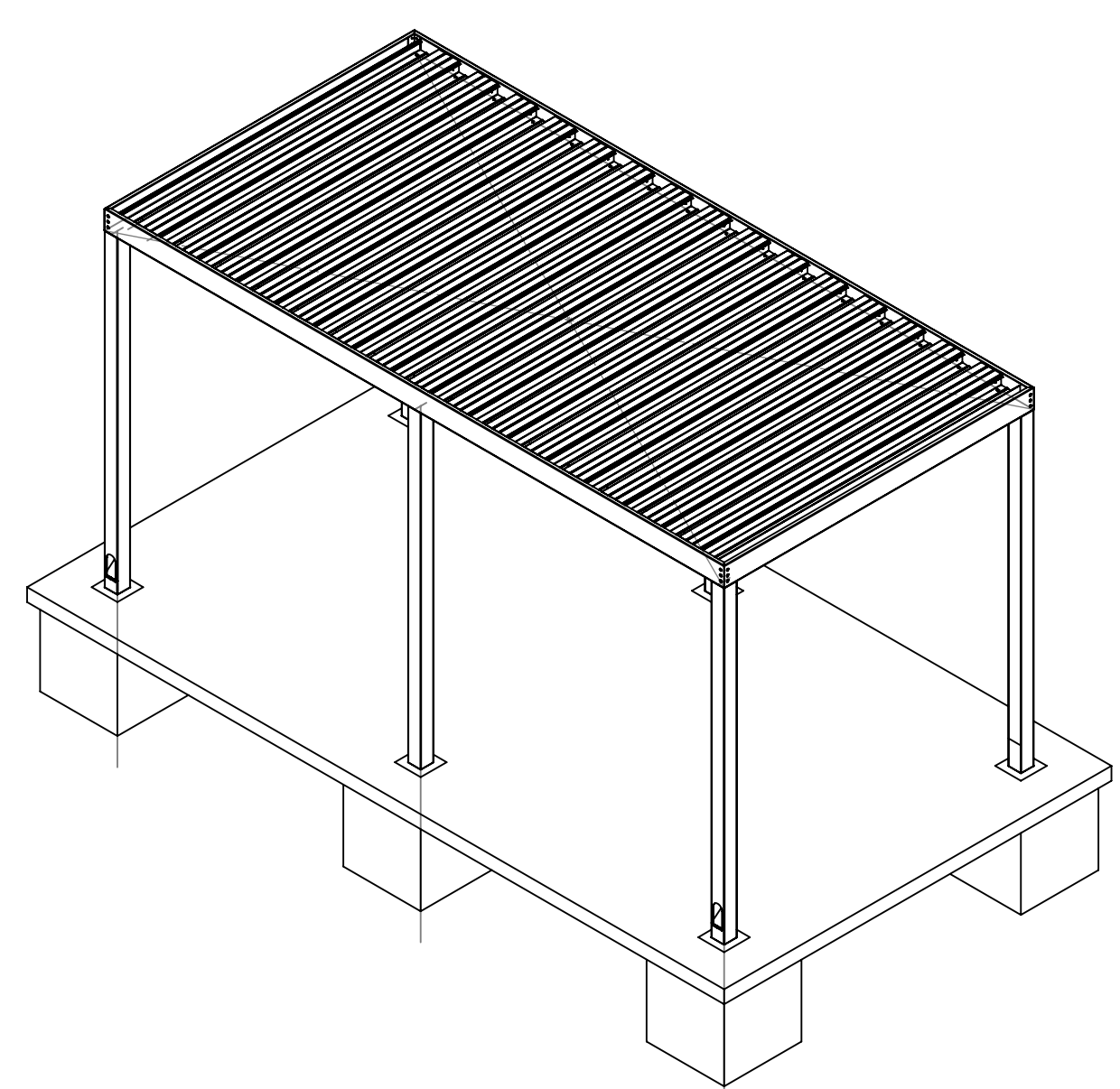
ISOMETRIC VIEW OF CANOPY
