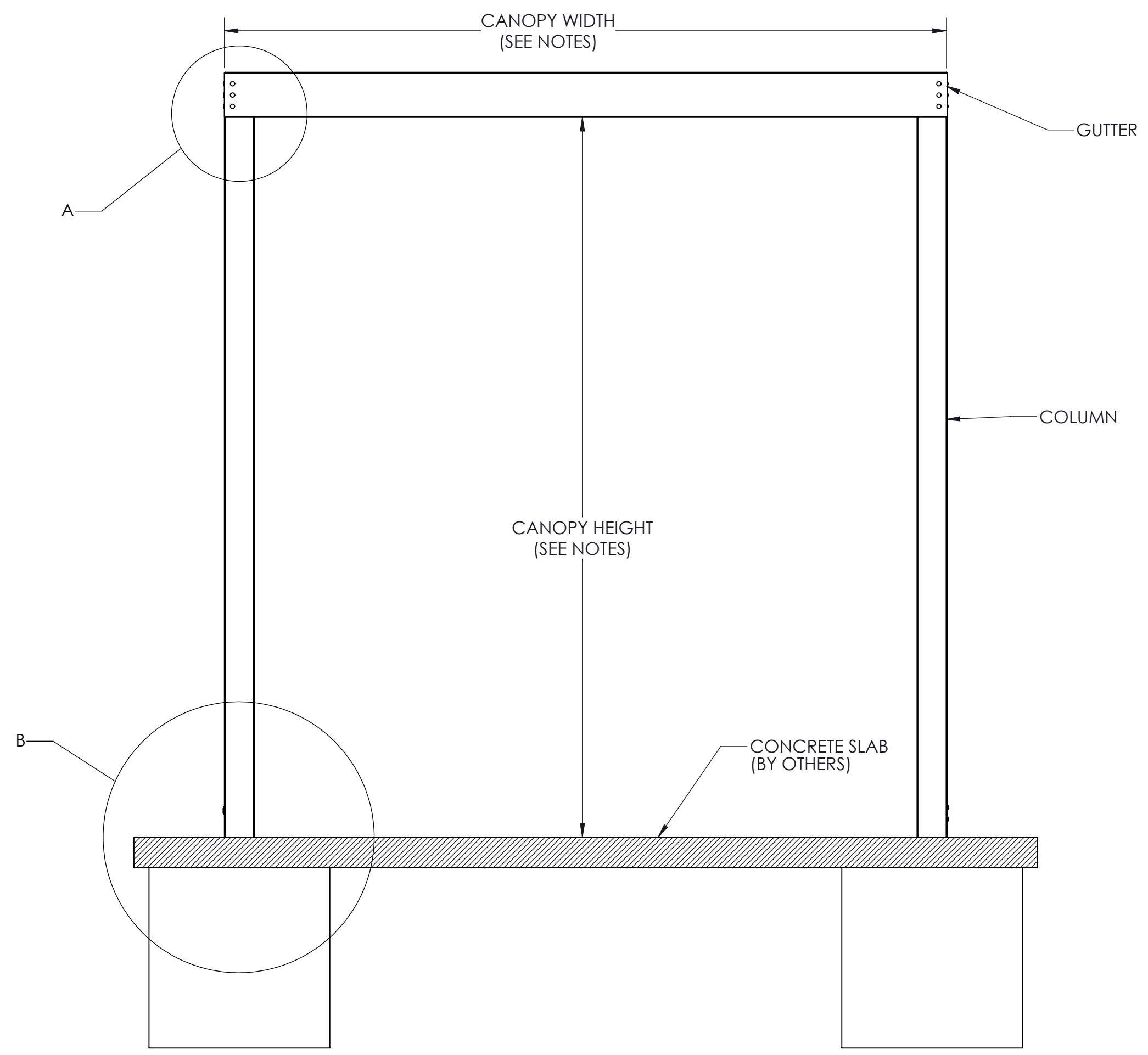
SECTION VIEW OF CANOPY
