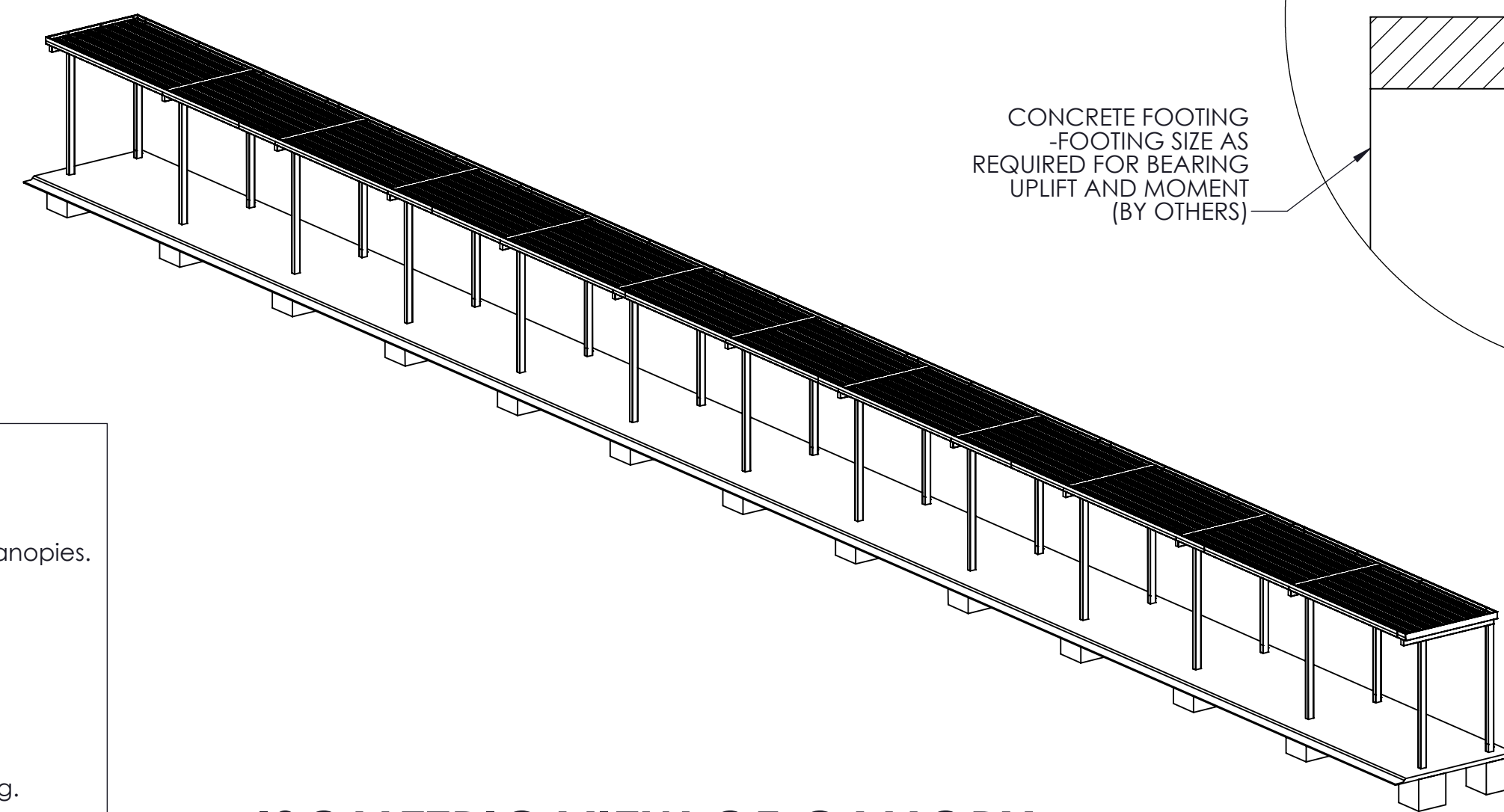
ISOMETRIC VIEW OF CANOPY
