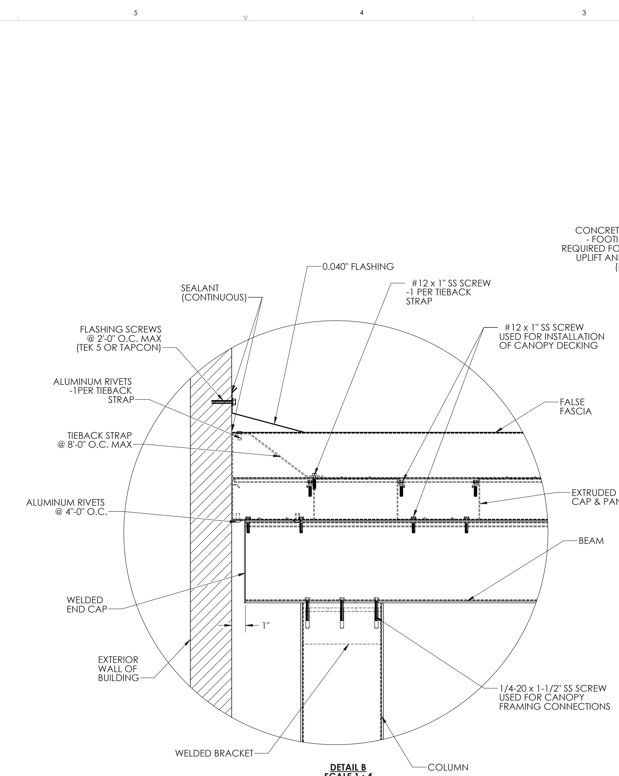
DETAIL B SCALE 1:4
