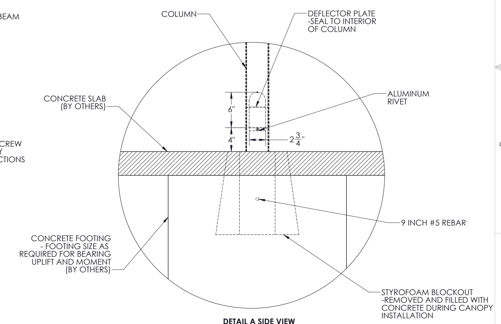
DETAIL A SIDE VIEW SCALE 1:8
