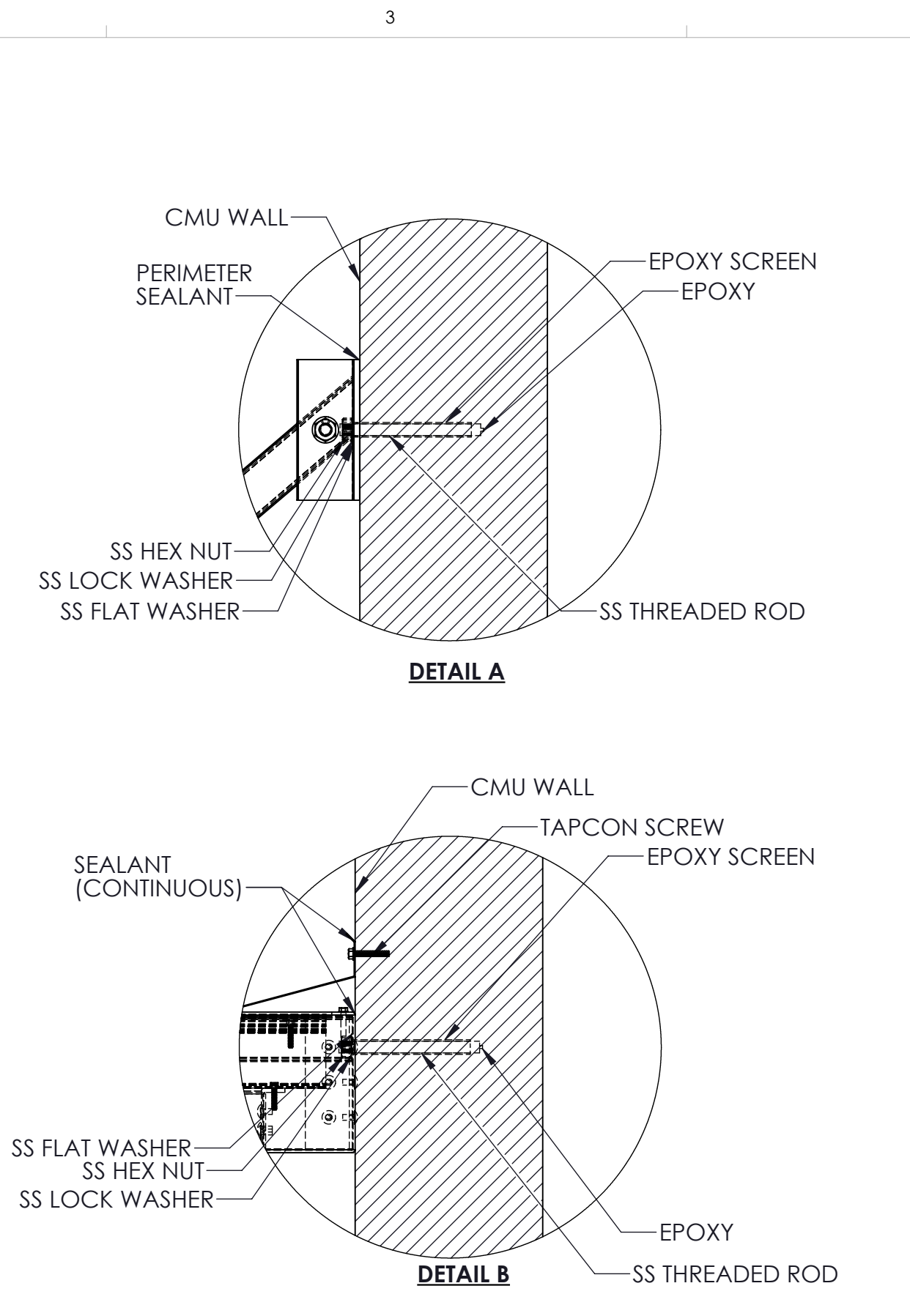
CMU Wall (Epoxy Anchors)
