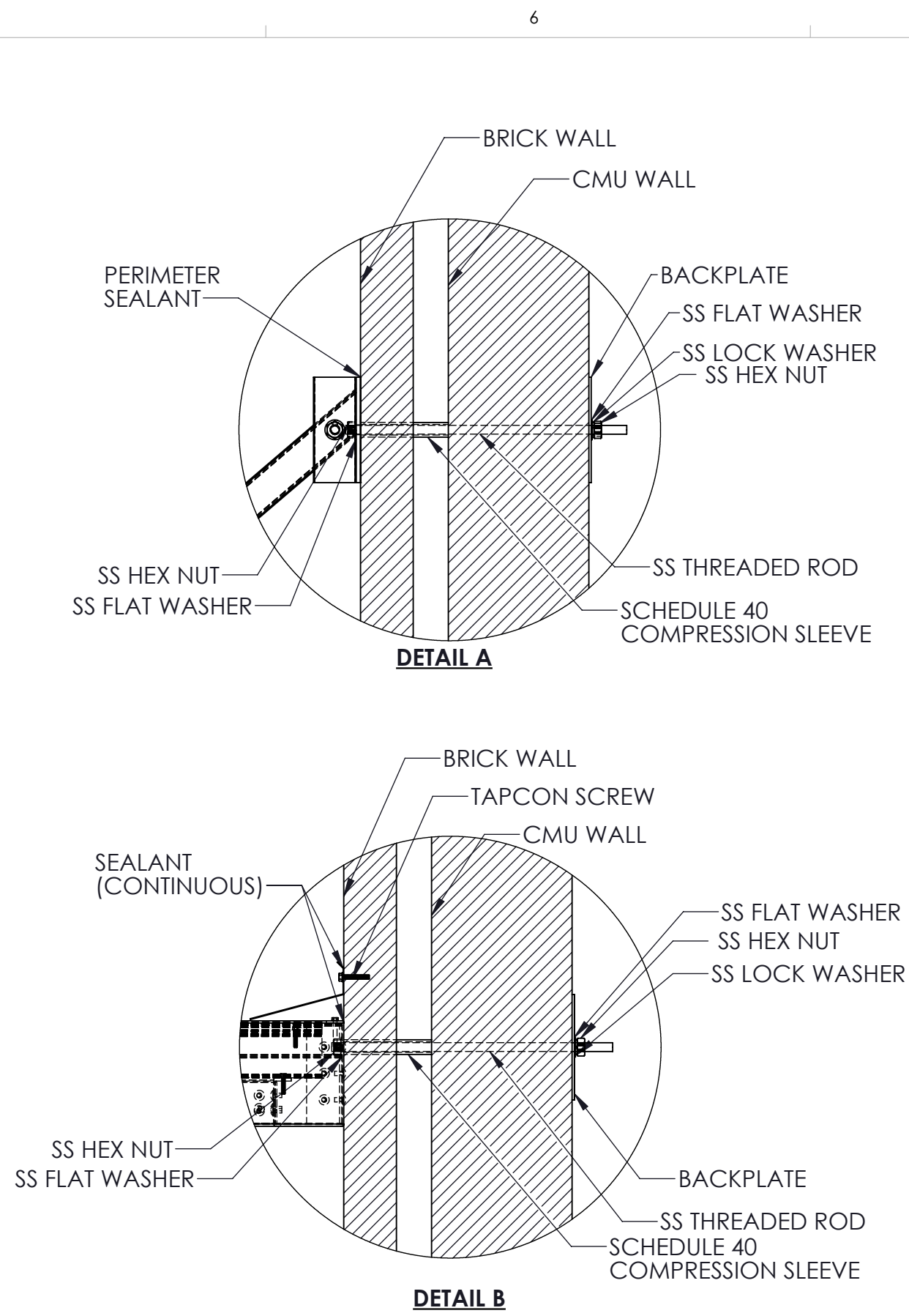
Brick and CMU Wall (Through Bolts)
