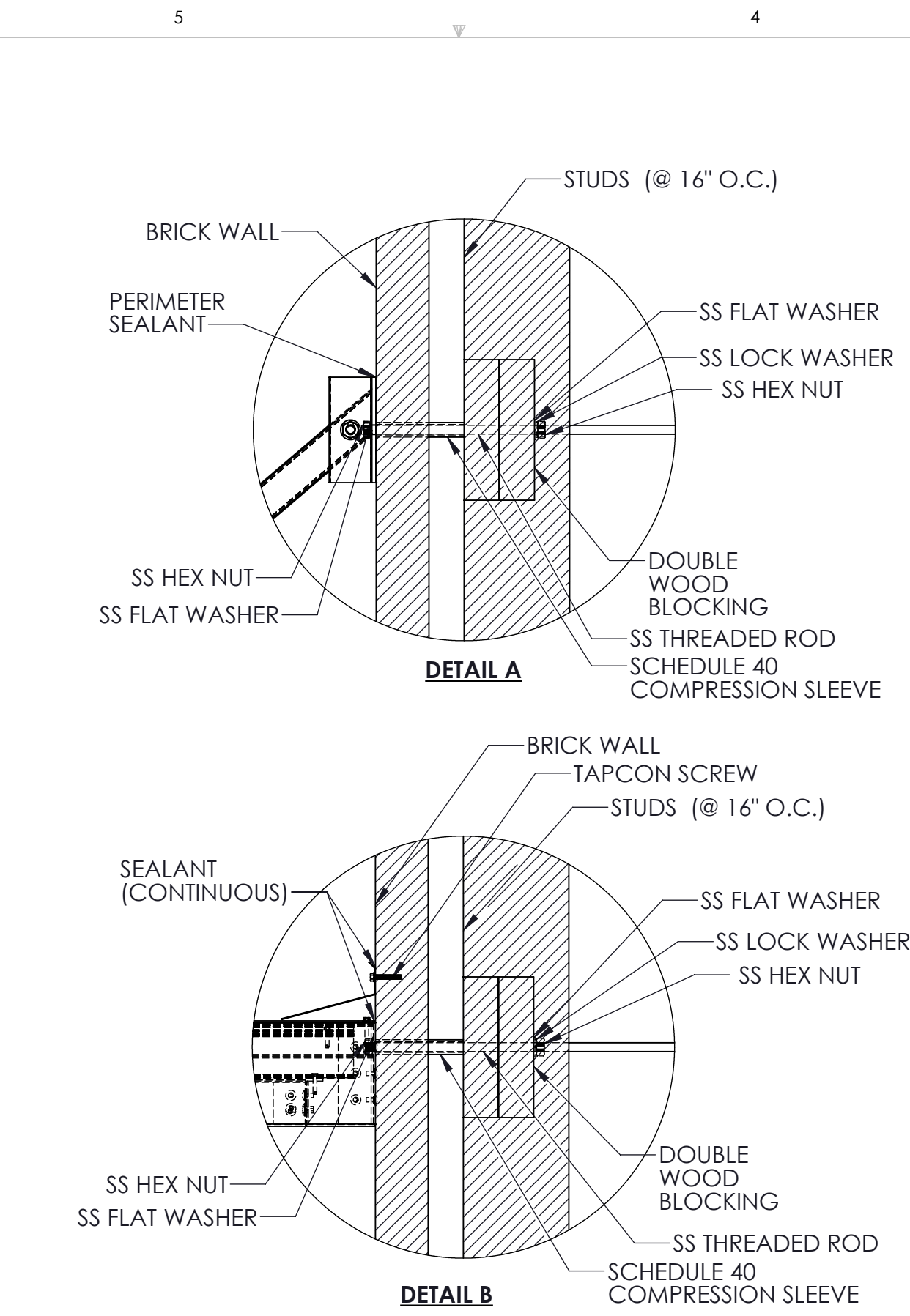
Brick Wall with Studs (Through Bolts)
