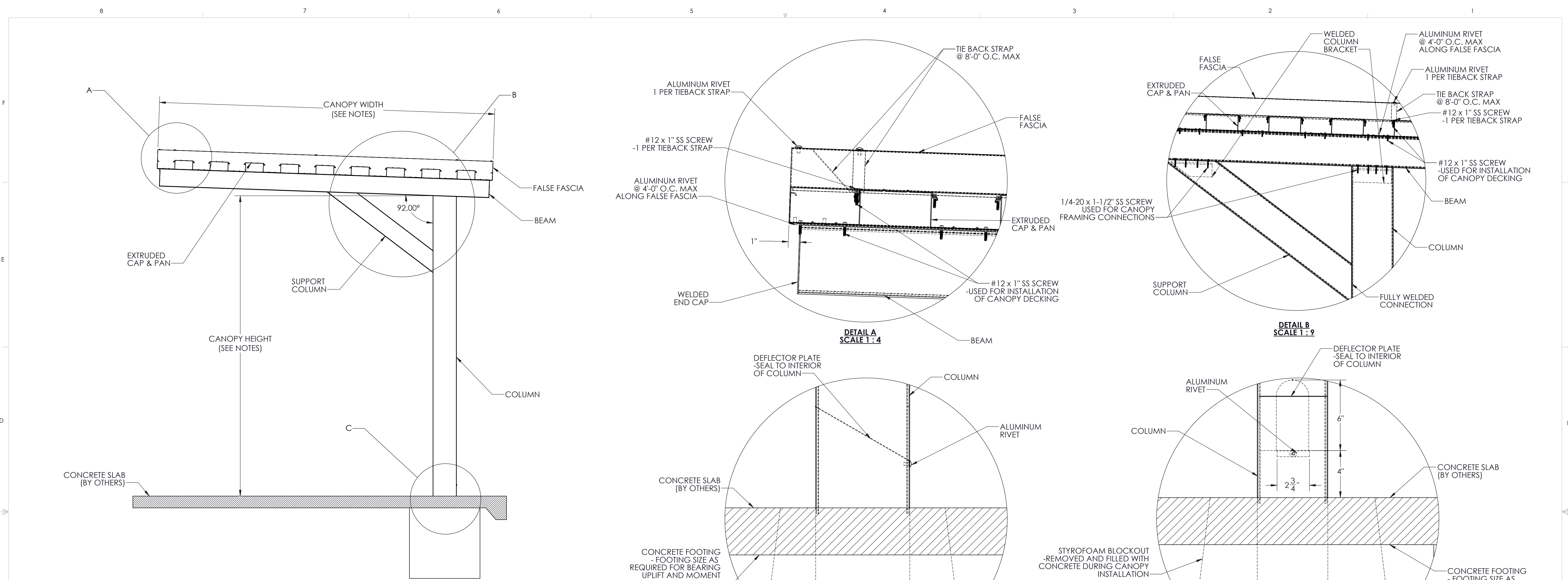
SECTION VIEW OF CANOPY
