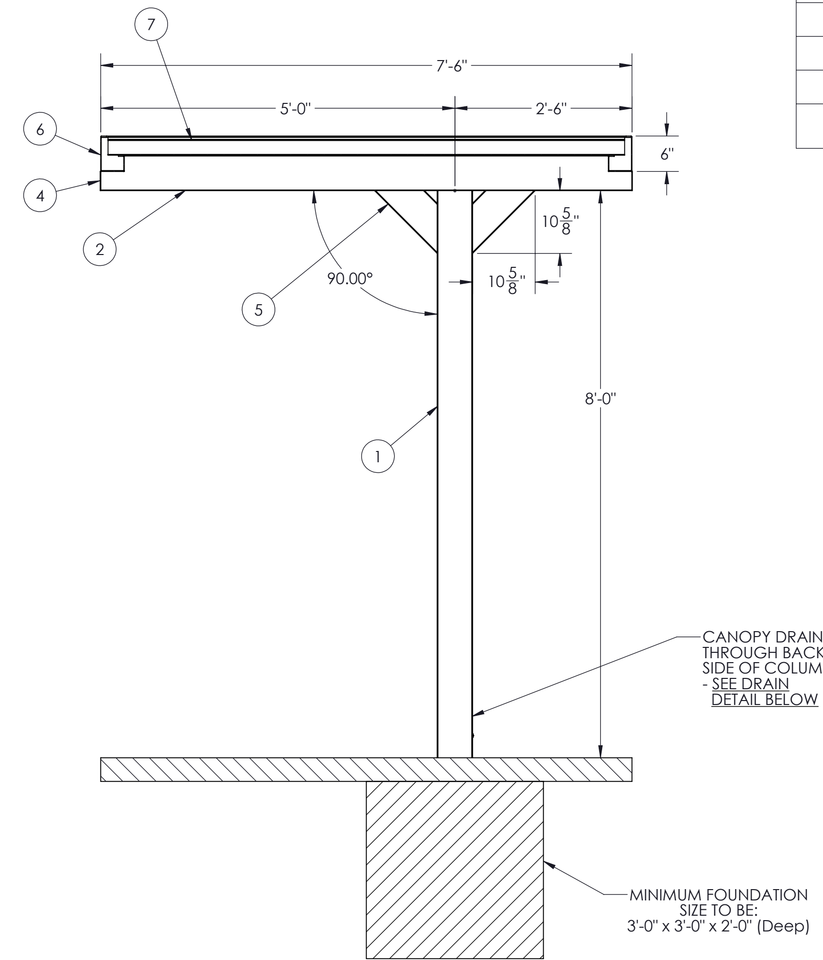
SECTION A-A SCALE 1 : 16 SECTION VIEW
