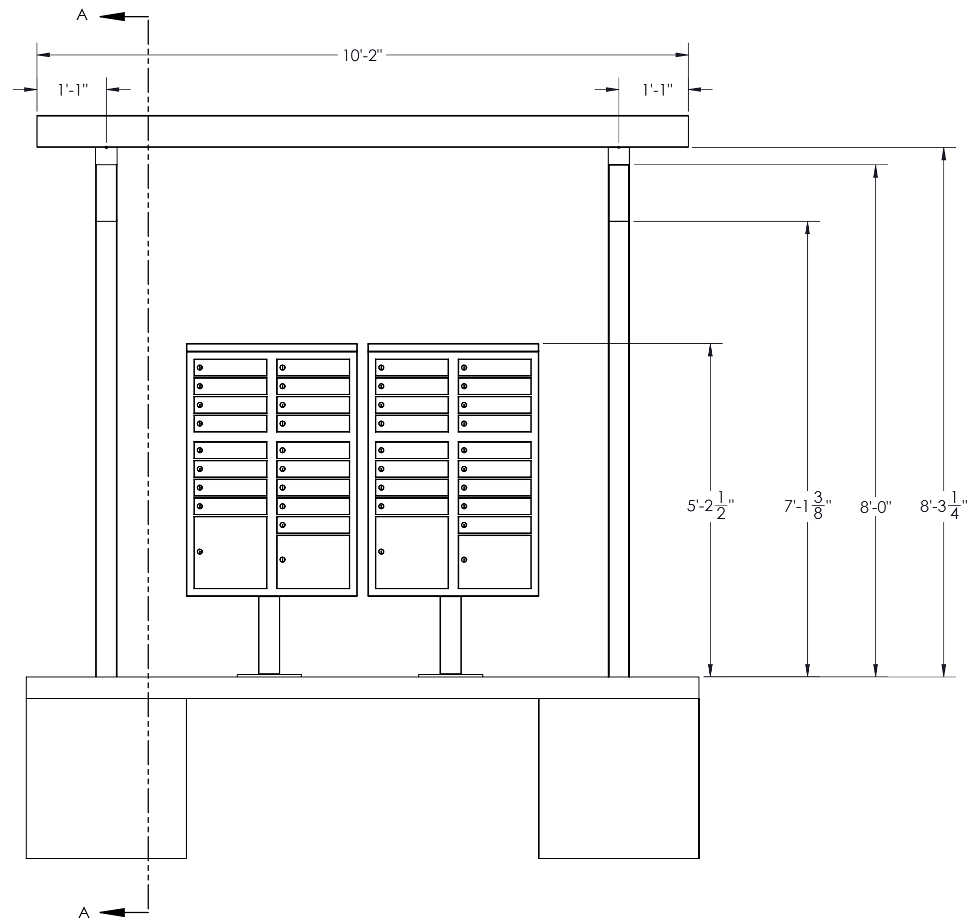
ELEVATION VIEW
