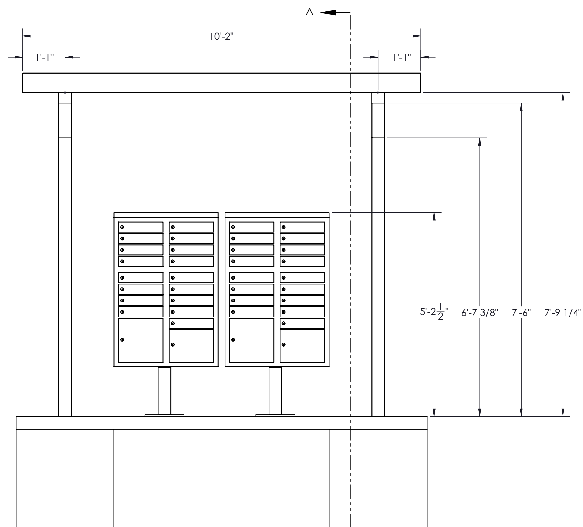
ELEVATION VIEW
