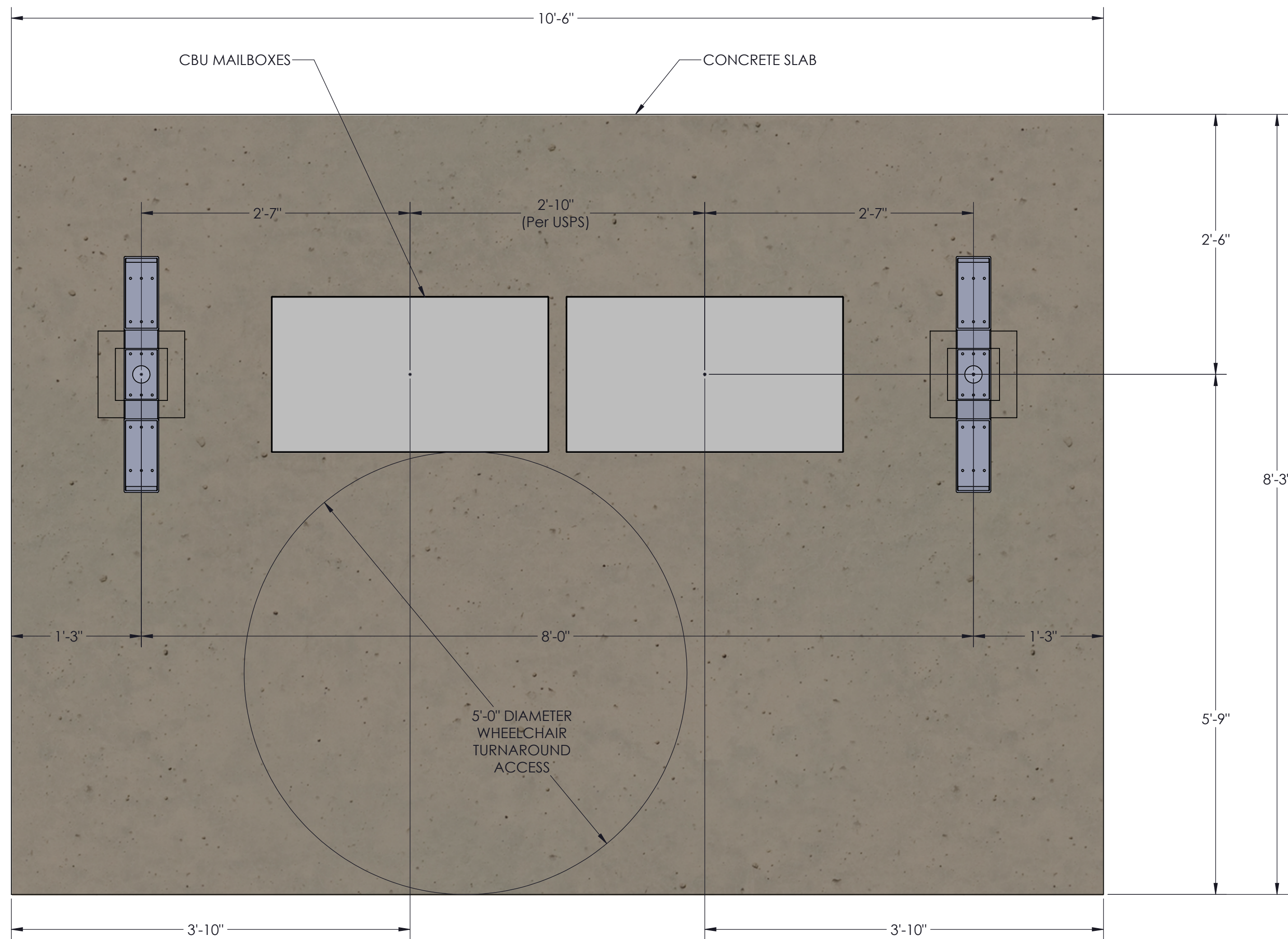
TOP VIEW
