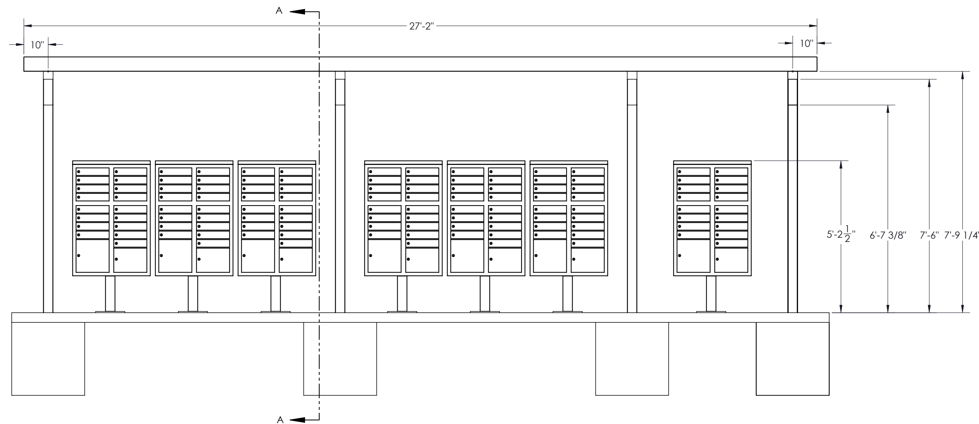
ELEVATION VIEW
