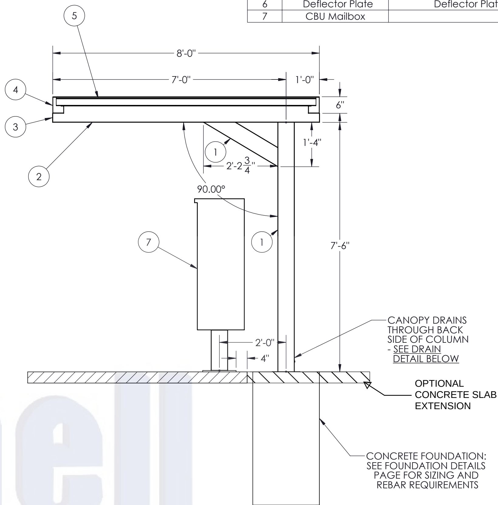
SECTION A-A SCALE 1 : 21 SECTION VIEW
