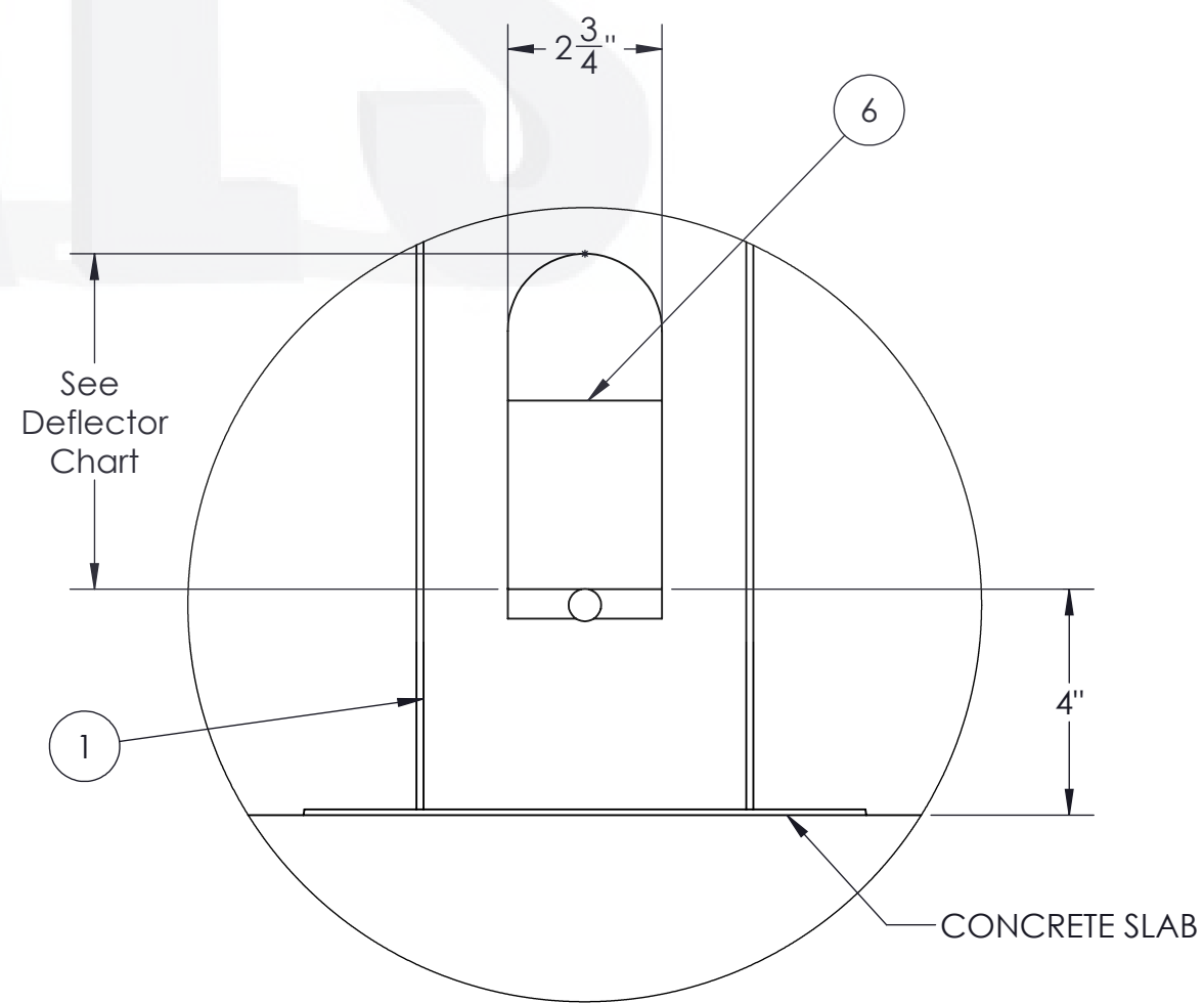
COLUMN DRAIN HOLE DETAIL SCALE 1 : 3.5
