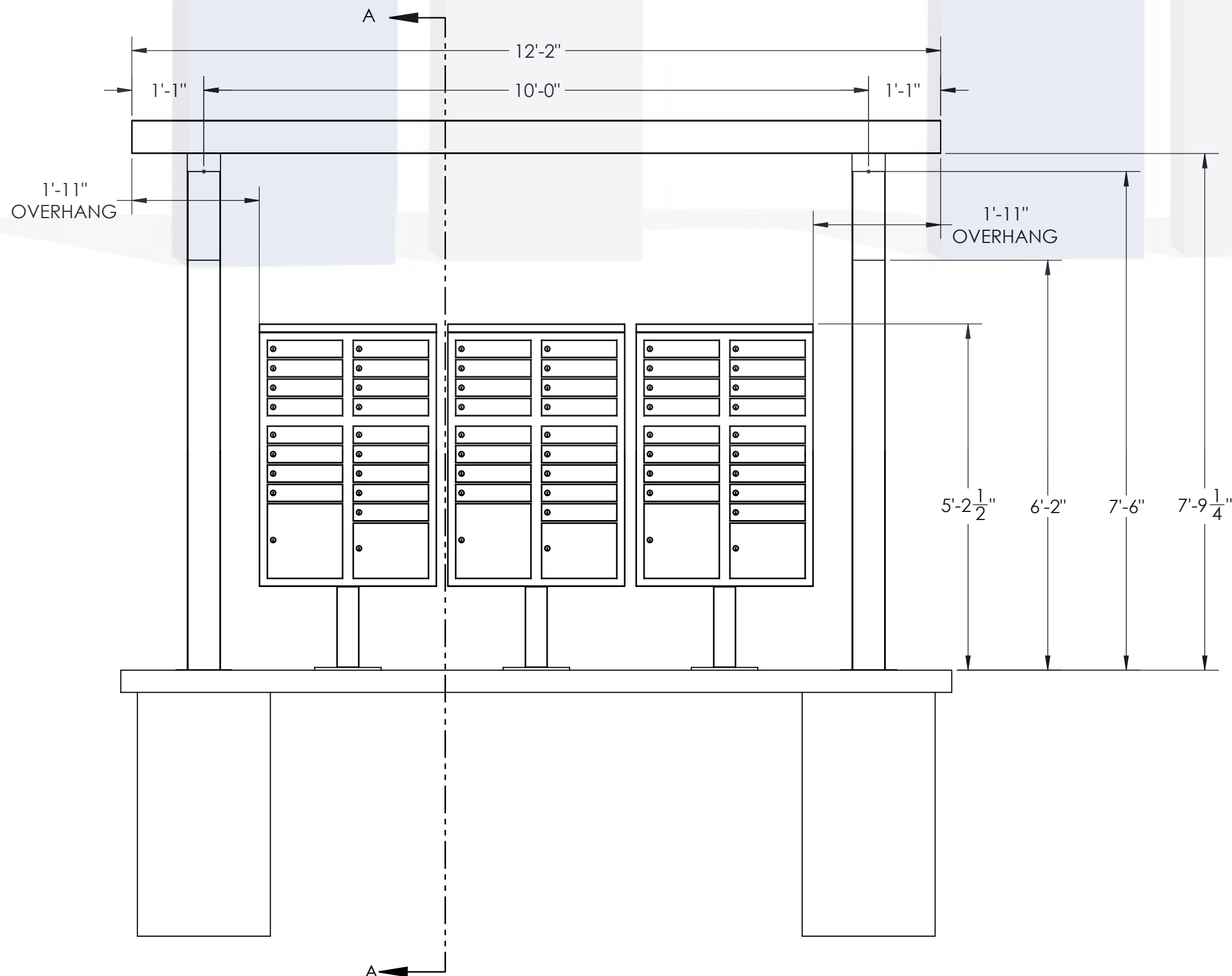
ELEVATION VIEW
